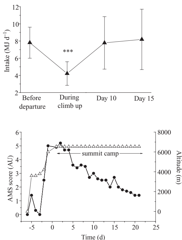
Figure 2 Energy intake (upper panel) and score for acute mountain sickness (AMS, lower panel) in 10 subjects during a 21-day stay at 6,524 m. * significantly different from the other time point ( P < 0.001 ) (from Westerterp et al. (79)). \Delta , altitude in meters; \bullet , Lake Louise AMS score in arbitrary units.
